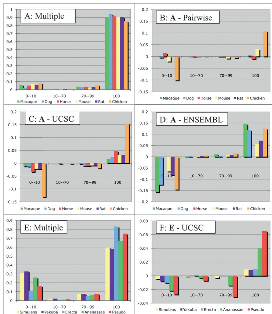
Figure 4. Exon alignment accuracy for vertebrate (A–D) and Drosophila (E,F) genomes. Each category on the X-axis shows the exons for a particular species that are aligned to a reference genome exon over the given fraction of their length. The Y-axis for A and E shows the overall fraction of exons in each category for our alignments, while the other plots show the difference of these fractions between our multiple alignments and those from the UCSC Genome Browser (ours minus UCSC, C and F), those from the Ensembl browser (D), and our pairwise alignments (B). Our algorithms align more exons perfectly (100% category) and fewer exons are not aligned at all (0–10 category) for all species. In the comparison between our multiple and our pairwise alignments, while the macaque alignments are identical, and the dog alignments are nearly identical (the two species are close), the human/mouse alignment is slightly improved, and nearly 10% of chicken exons were aligned in the multiple but not pairwise alignment. The 23-way Ensembl alignments that we used had a different version of the horse genome, preventing a direct comparison, and we did not generate a pairwise human/rat alignment (rat would be very similar to mouse), hence the missing columns in B and D.
