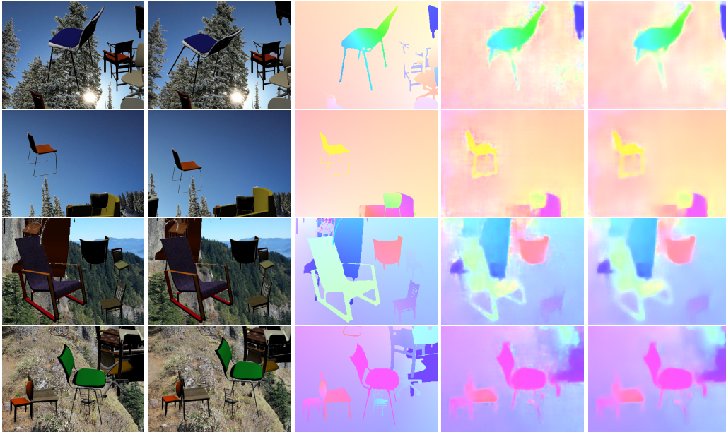
Figure 5: Optical flow : Left to right: first and second input, ground-truth, Flownet [12], ours.
