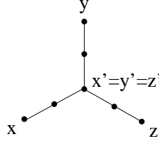
Figure 2.3: Illustration of Corollary 1
