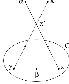
Figure 3.1: Illustration of Claim 8.
