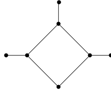
Figure 2.4: A diametral path graph that is not HDP.
