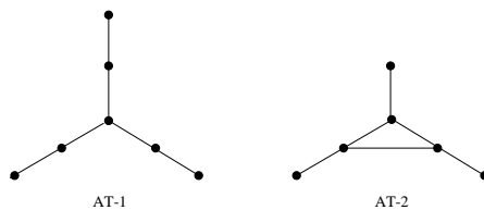
Figure 2.1: The minimal forbidden subgraphs for chordal diametral path graphs.
