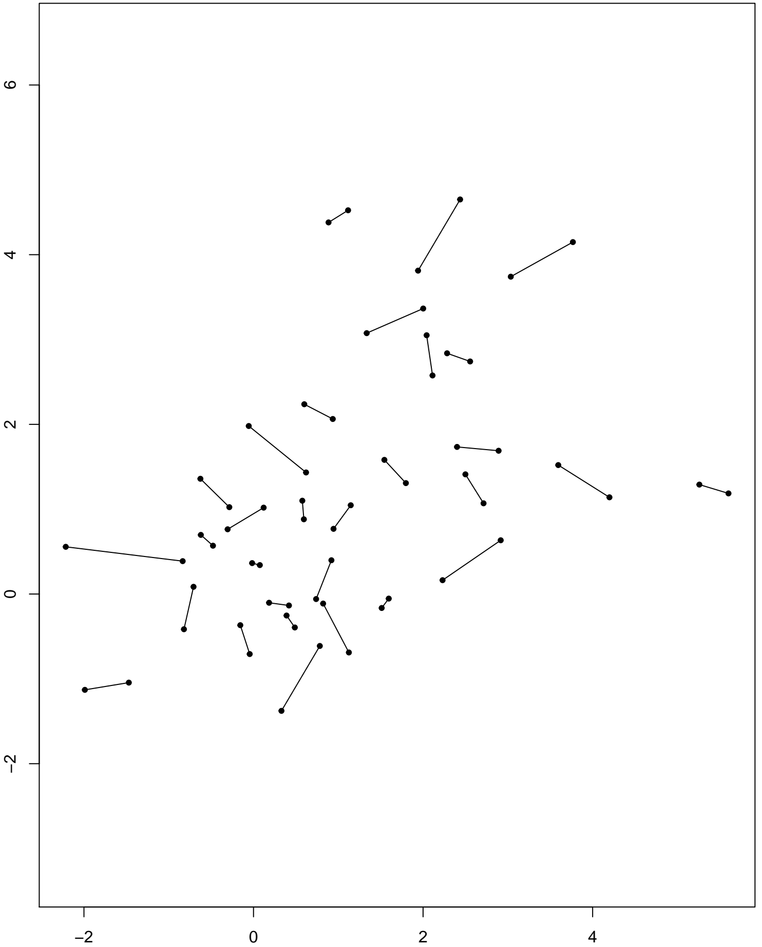
Seed 1, Total distance 15.1868
