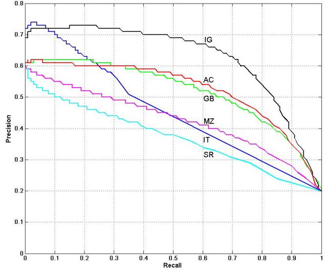
Figure 5. Precision-recall curve for naïve thresholding of saliency maps. Our method IG is compared against the five methods of IT [16], MZ [22], GB [10], SR [12], and AC [1] on 1000 images.
