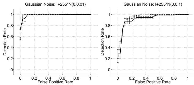
Fig. 9. Gaussian noise changes. Solid line represents the phase-based feature. Dotted line represents differential invariant feature.
