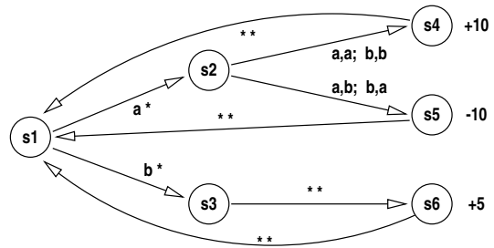
Figure 1: A Simple MMDP with a Coordination Problem.
