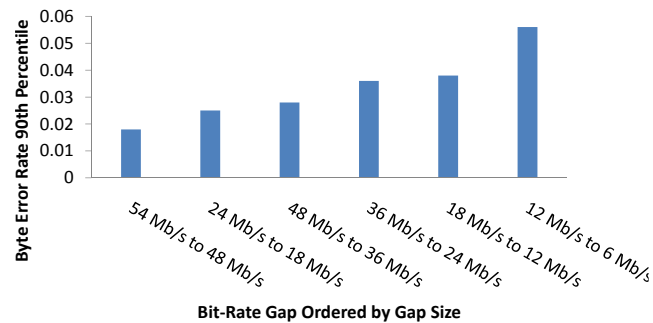
Figure 4: Byte Error vs. Gap Size: Byte error rates in partial packets increase with the size of the gap between the used bit-rate and the one below it.
