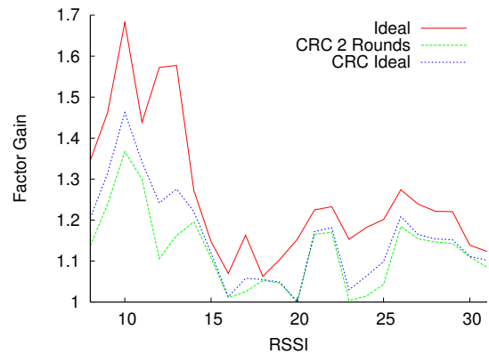
Figure 12: Effectiveness of the per block CRC schemes in harnessing partial packets: The figure shows that an idealized per block CRC scheme captures about 60% of the ideal gains available from partial packets, whereas a more realistic 2-round CRC-based scheme obtains 50% of these gains.
