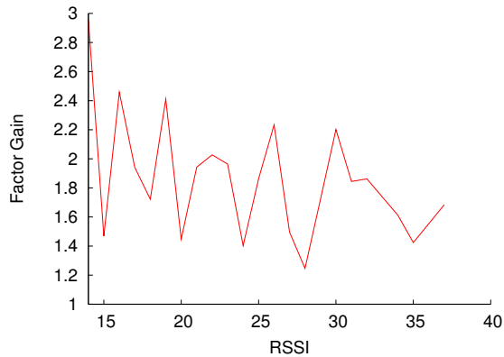
Figure 20: ZipTx’s throughput gain in mobile channels: As a result of autorate’s difficulty in picking a good rate, ZipTx improves the throughput by up to 3x, when moving at a walking pace.
