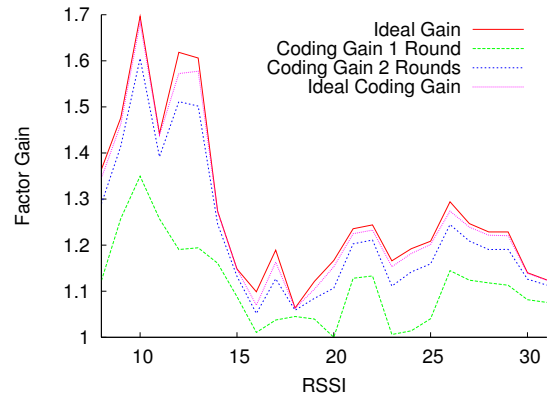
Figure 16: Efficacy of a coding scheme at harnessing partial packets: This shows that a coding-based scheme can harness most of the potential gain of partial packets. Further, it can do so with just two rounds of redundancy.
