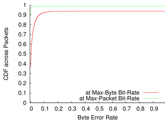
Figure 3: CDF of byte error rates in typical 802.11 channels: The figure plots the byte error rate for when the autorate algorithm maximizes the correct-packet throughput, as in today’s networks, and when it maximizes the correct-byte throughput.
