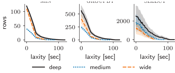
Fig. 10. Number of rows sent over the network for each types of queries across a range of laxity values. Shaded areas show standard deviation.
