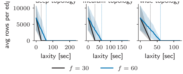
Fig. 11. Average number of rows accessed by each local edge replicas as a function of laxity for different with push period f = 30 seconds and f = 60 seconds. Feather shifts work from edges towards the core and cloud nodes, and once L > f edges are seldom involved in answering global queries. Shaded areas show standard deviation. Dotted vertical lines show push period f .
