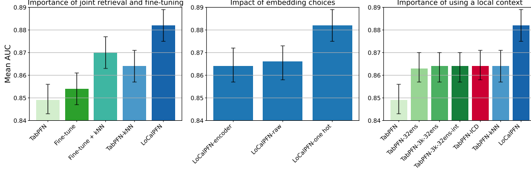
Figure 10: Ablations on Small Datasets
