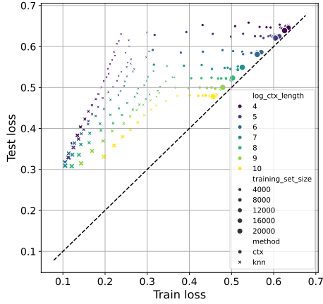
(c) electricity
