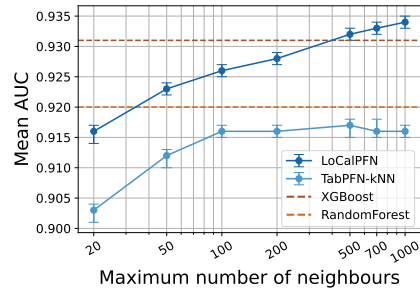
Figure 6: Ablating max # of neighbours
