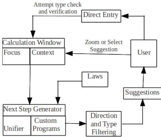
Fig. 1. Backbone
