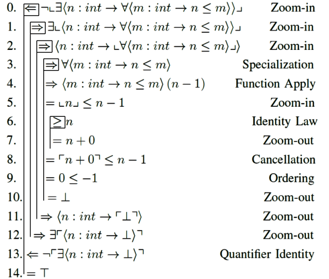
Fig. 3. Detailed Proof
