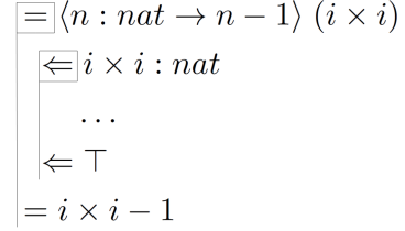
Fig. 5. Type Proof
