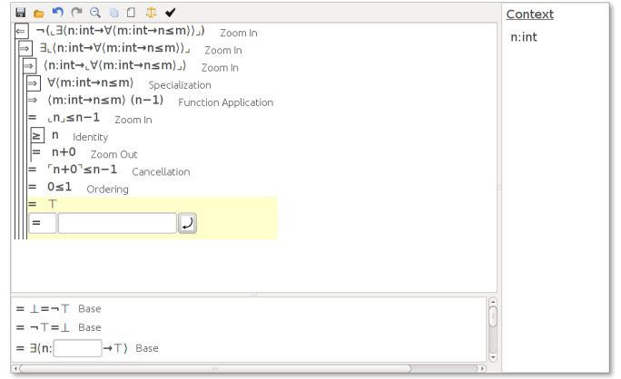
Fig. 2. Calculation Window
