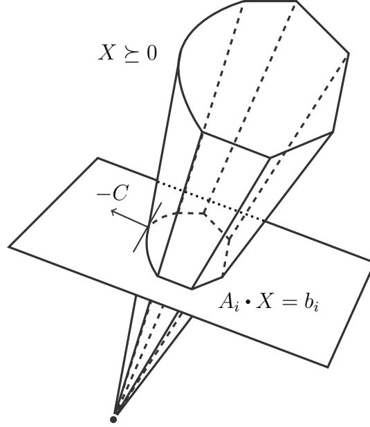
Figure 3.1: A semidefinite program minimizing C \cdot X over the spectrahedron formed from the intersection of the cone X \succeq 0 with the affine subspace A_i \cdot X = b_i for i \in [m] .
