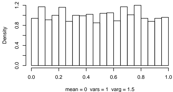
Histogram of 2000 p-values from standard t test
