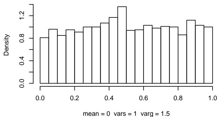
Histogram of 2000 p-values from modified t test
