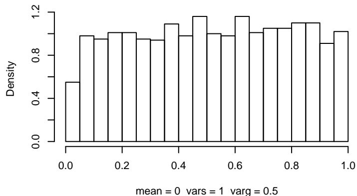
Histogram of 2000 p-values from modified t test
