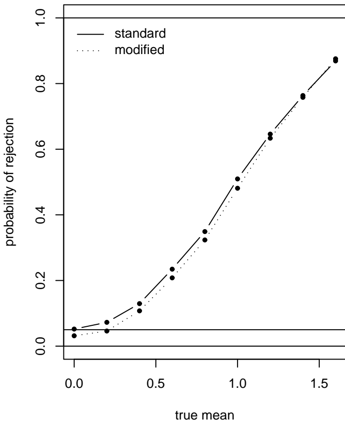
Rejection probabilities, vars = 1 varg = 0.5
