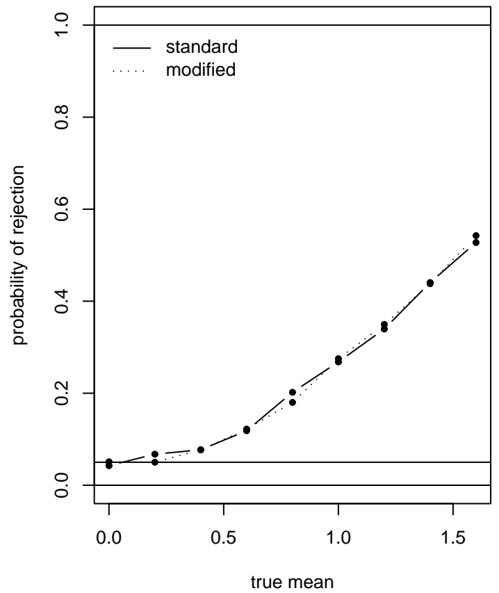
Rejection probabilities, vars = 1 varg = 1.5
