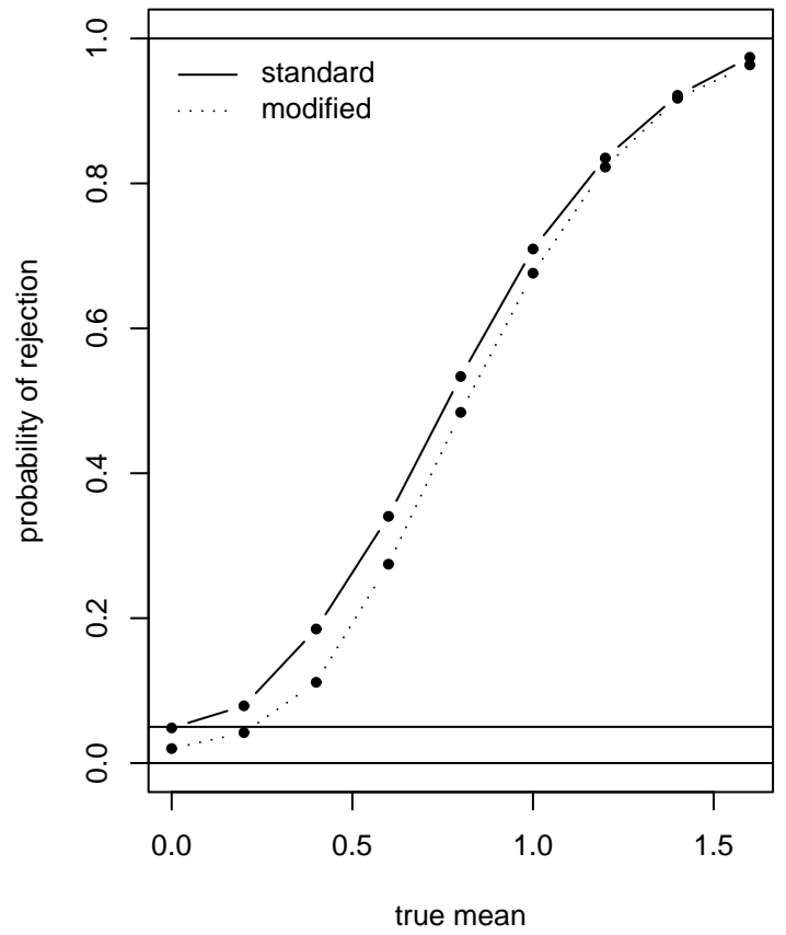
Rejection probabilities, vars = 1 varg = 0.2
