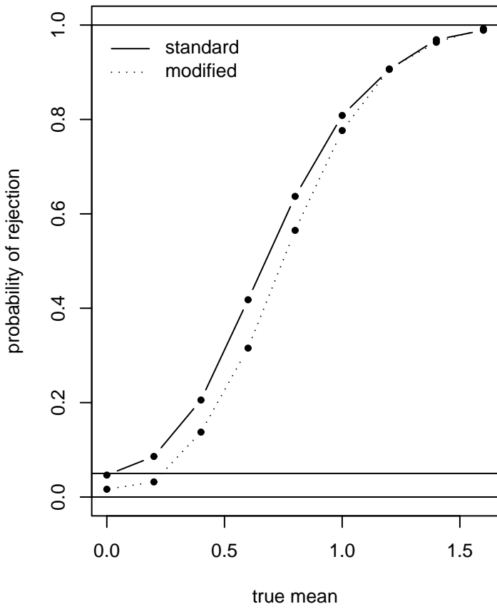
Rejection probabilities, vars = 1 varg = 0.1
