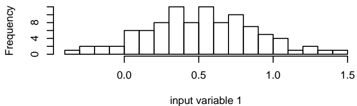
class 0
