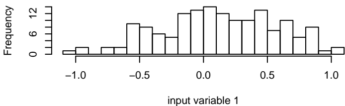
class 1
