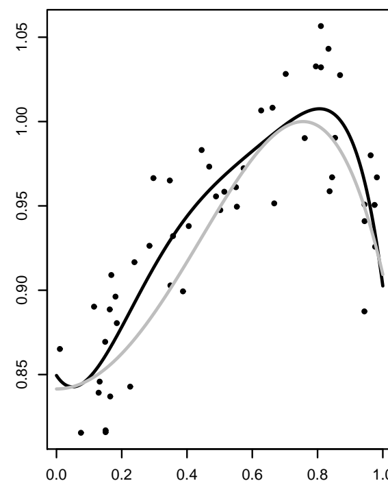
Gaussian basis function fit, s = 2.5
