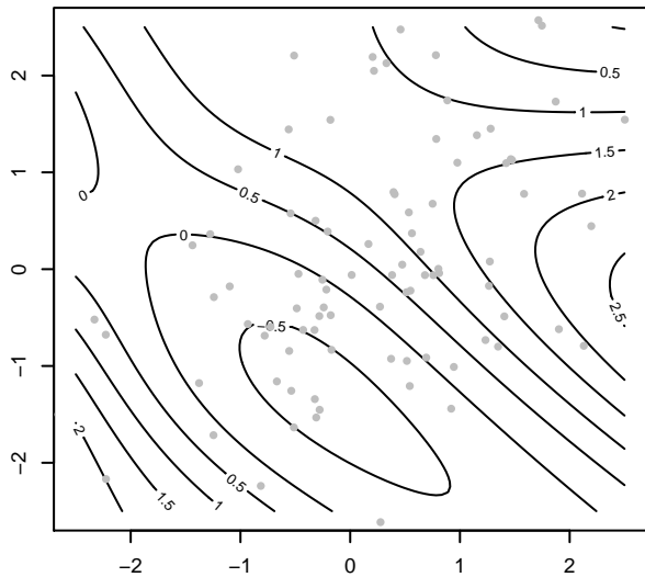
Function learned by network, and training points
