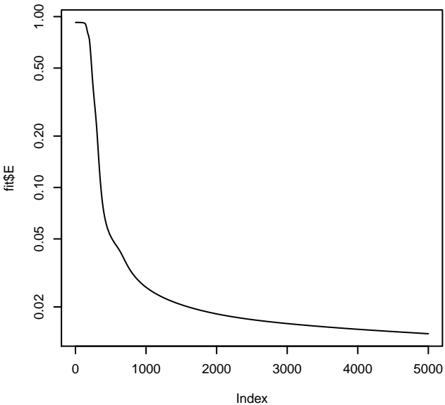
Training error
