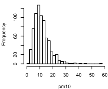
Histogram
