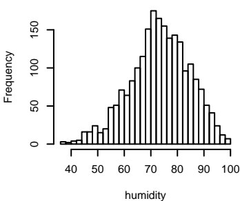
Histogram
