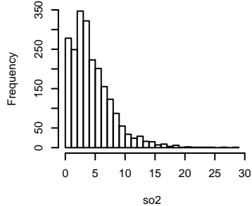
Histogram
