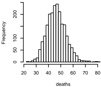
Histogram
