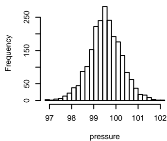
Histogram
