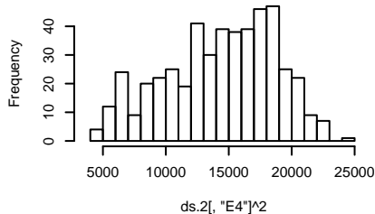
Histogram of ds.2[, "E4"]^2
