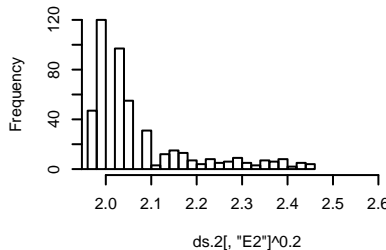
Histogram of ds.2[, "E2"]^0.2
