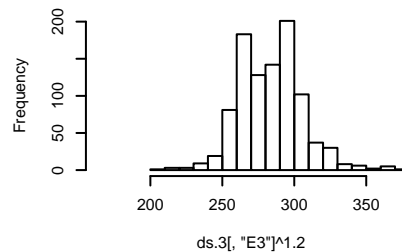
Histogram of ds.3[, "E3"]^1.2
