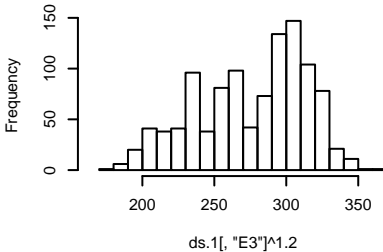
Histogram of ds.1[, "E3"]^1.2
