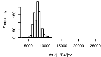
Histogram of ds.3[, "E4"]^2
