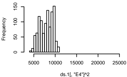
Histogram of ds.1[, "E4"]^2
