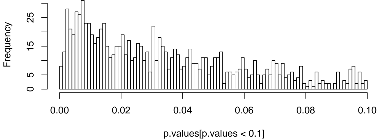
Histogram of p.values[p.values < 0.1]
