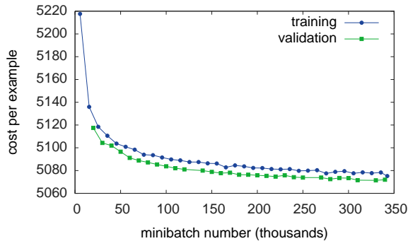
Figure 11. Training and validation cost on SVHN. The validation cost is consistently lower because the validation set patches were extracted from the image centre (rather than from random locations, as in the training set). The network was never able to overfit on the training data.
