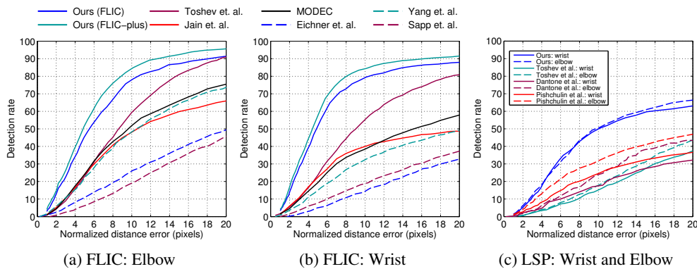
Figure 7: Model Performance
