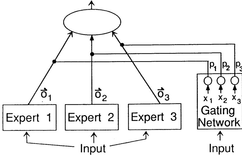
Figure 1: A system of expert and gating networks. Each expert is a feedforward network and all experts receive the same input and have the same number of outputs. The gating network is also feedforward and may receive a different input than the expert networks. It has normalized outputs p_j = \exp(x_j) / \sum_i \exp(x_i) , where x_j is the total weighted input received by output unit j of the gating network. p_j can be viewed as the probability of selecting expert j for a particular case.
